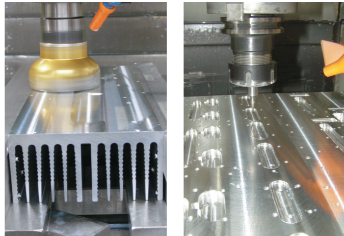
CNC machining
